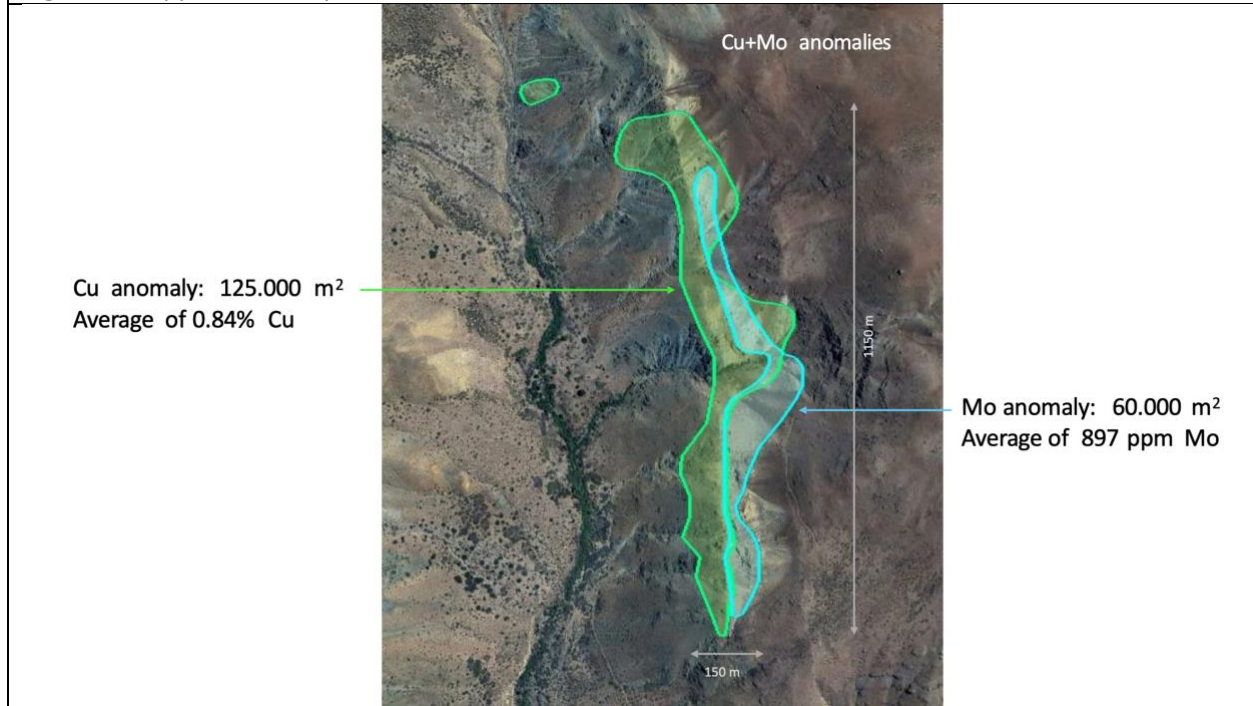
Figure 2. Copper and molybdenum anomalies associated with the PFZ, South Caballos, Chile
