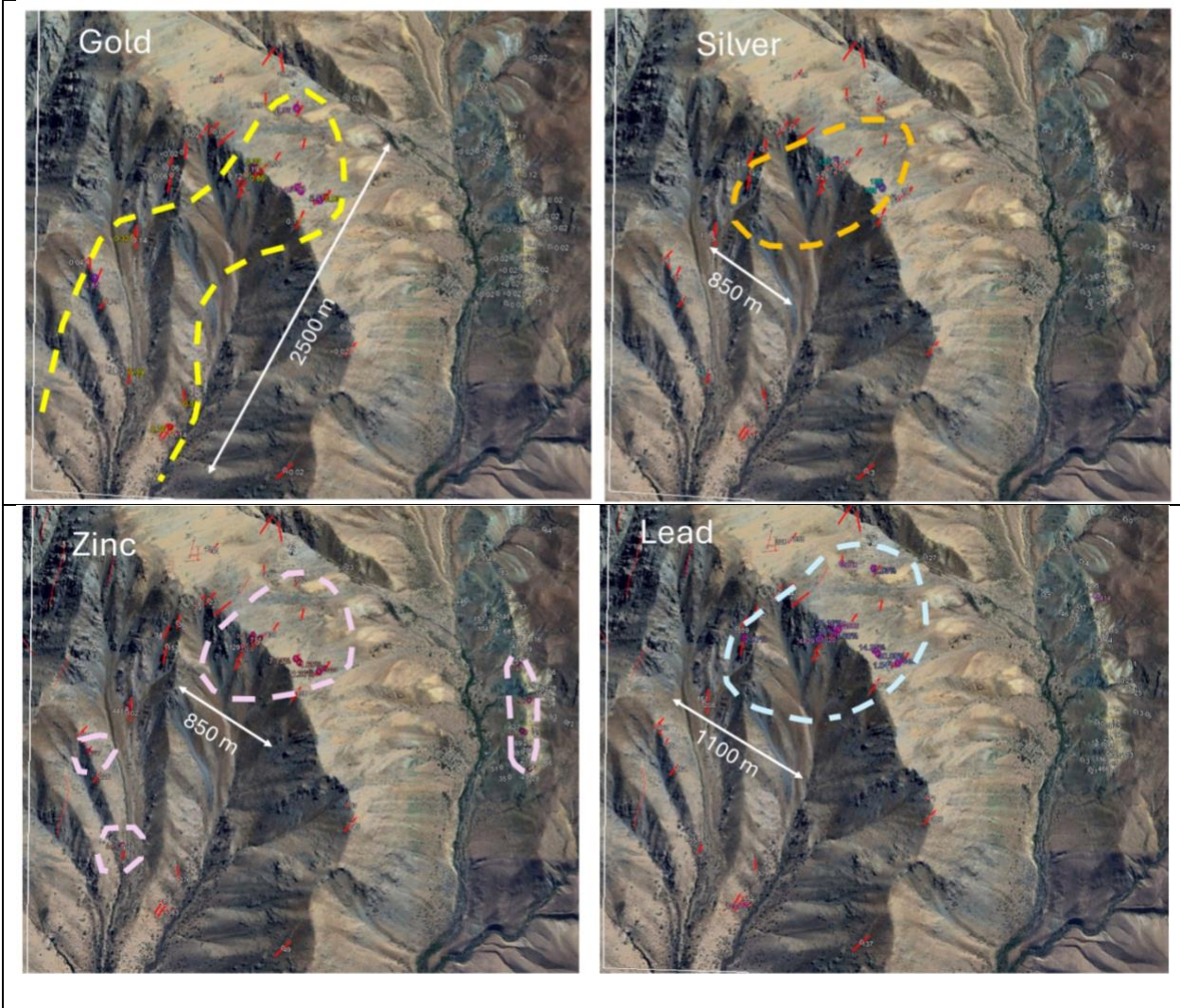
Figure 3. Gold, silver, zinc, and lead anomalies from veins west of the PFZ, Southern Caballos, Chile
